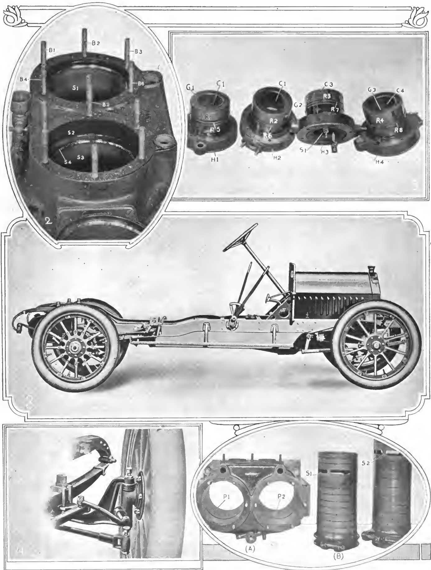
Fig. 2—Showing one pair of cylinders with the sleeves in place and the heads removed indicating the condition of the bearing surfaces at the expiration of the test Fig. 3—Looking at the right-hand side of the Stearns-Knight chassis Fig. 4—Looking at the front axle, showing the method of construction Fig. 5—Showing the four cylinder heads as they were taken off the motor and the condition of the junk rings and other wearing surfaces at the time Fig. 6—Showing one pair of cylinders and one pair of sleeves and the condition of the surfaces at the expiration of a test run
